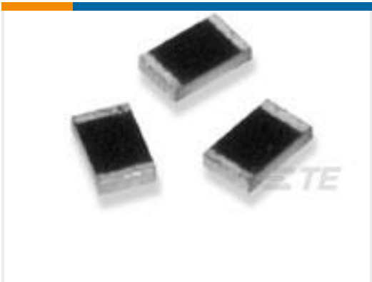
TE Part #1879278-2 RP 2A 28K 0.1% 15PPM 1K RL
