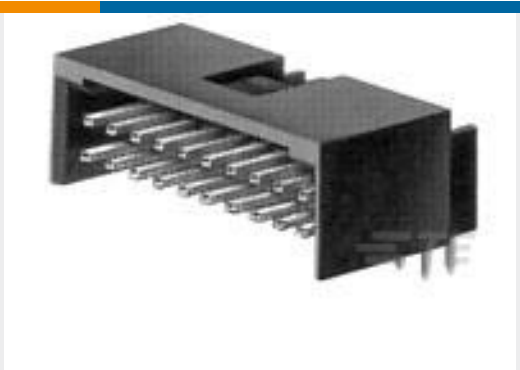
TE Part #103165-1 10 MODII HDR DRRA 3 /4SHRD .100
